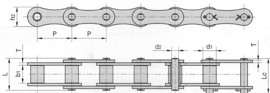
Rollenkette 208B RSC
