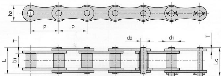
Rollenkette 208B RSC
