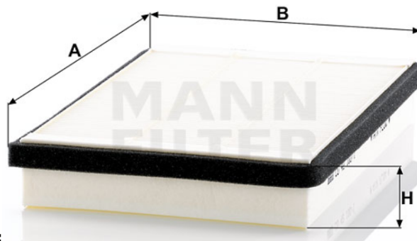
Kabinenfilter H931.812.140.511
