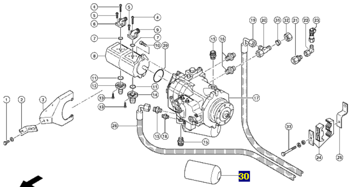
Hydraulikfilter 068959.0 CLAAS
