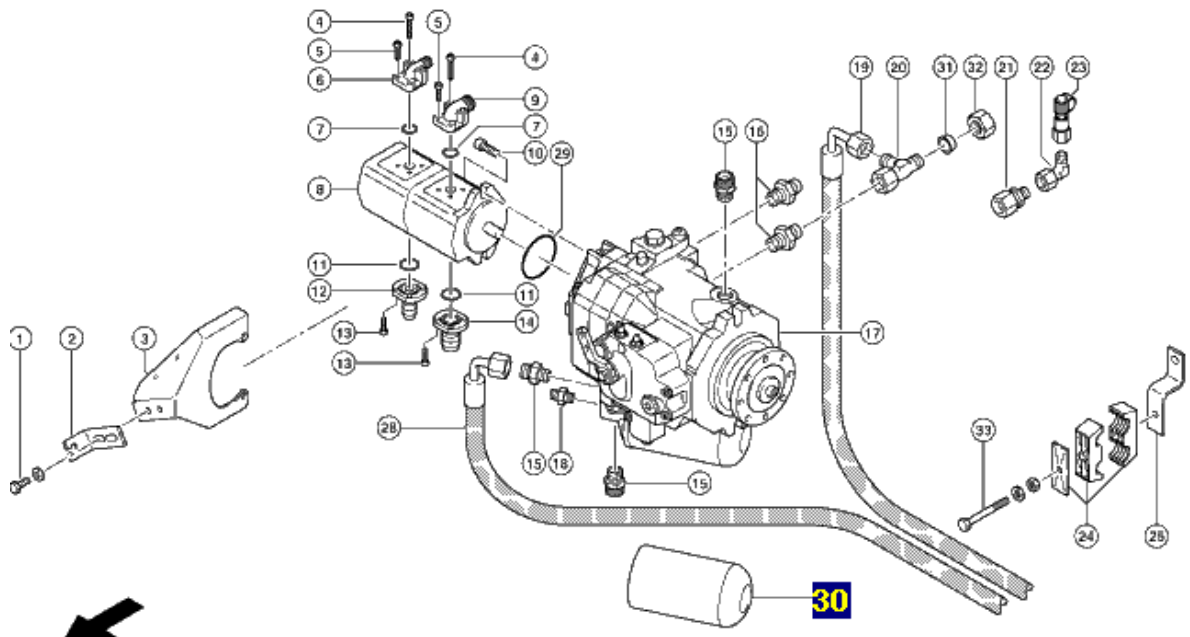
Hydraulikfilter 068959.0 CLAAS
